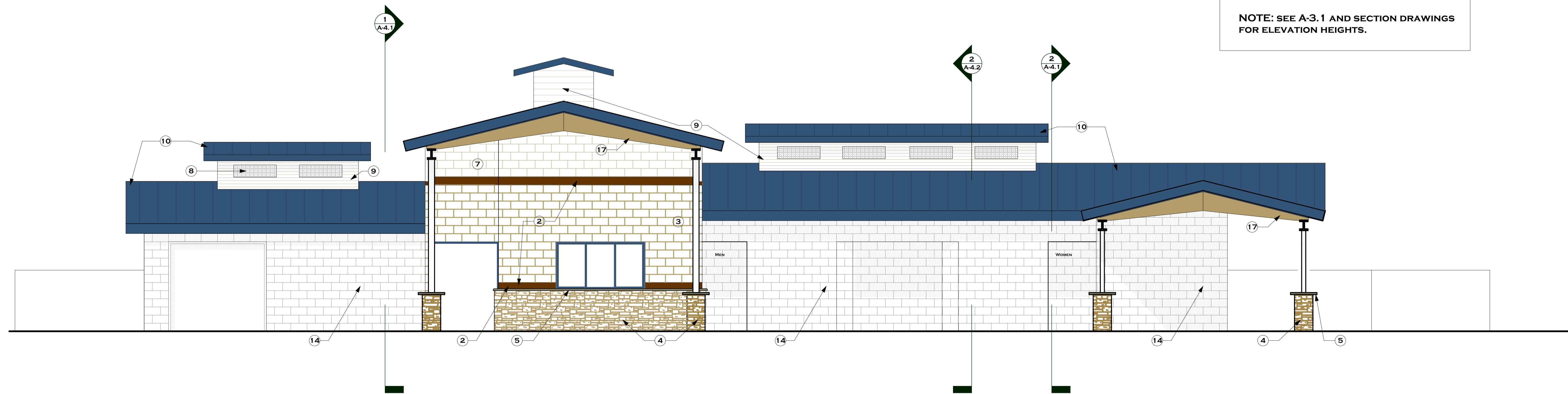
POOLSIDE (EAST) ELEVATION 1/4" = 1'-0"
