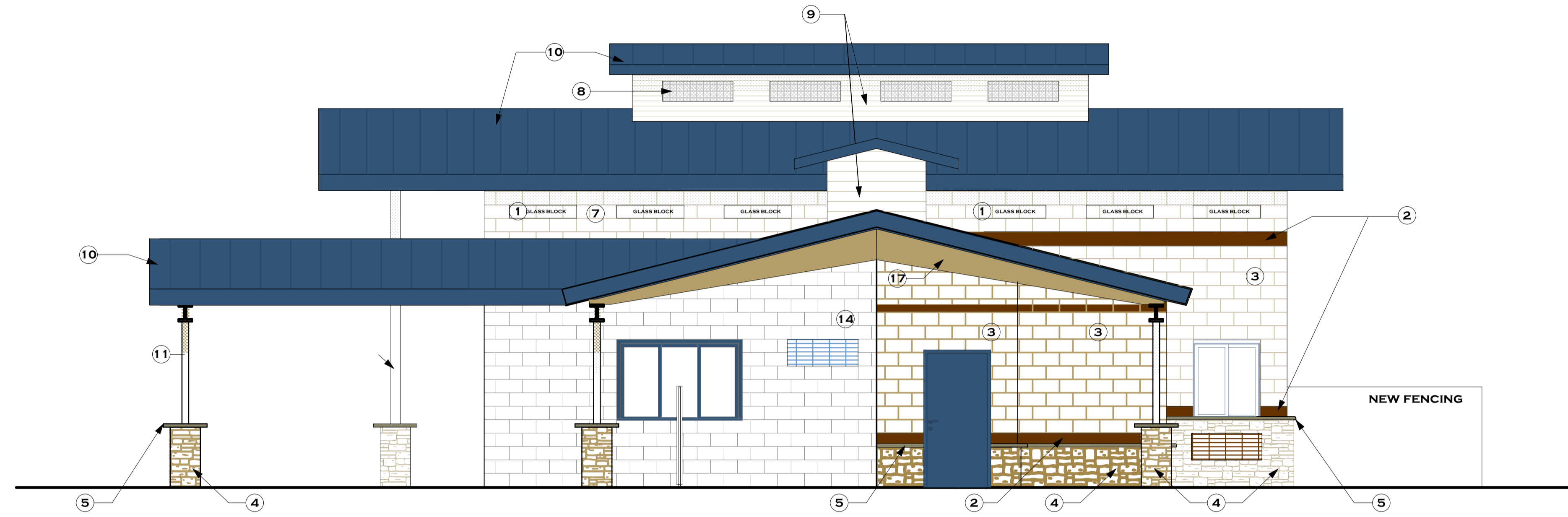
CONCESSIONS (NORTH) ELEVATION 1/4" = 1'-0"
