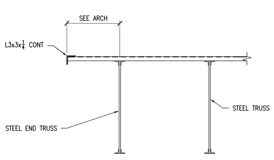
SECTION 11 3/4"=1'-0" S-4
