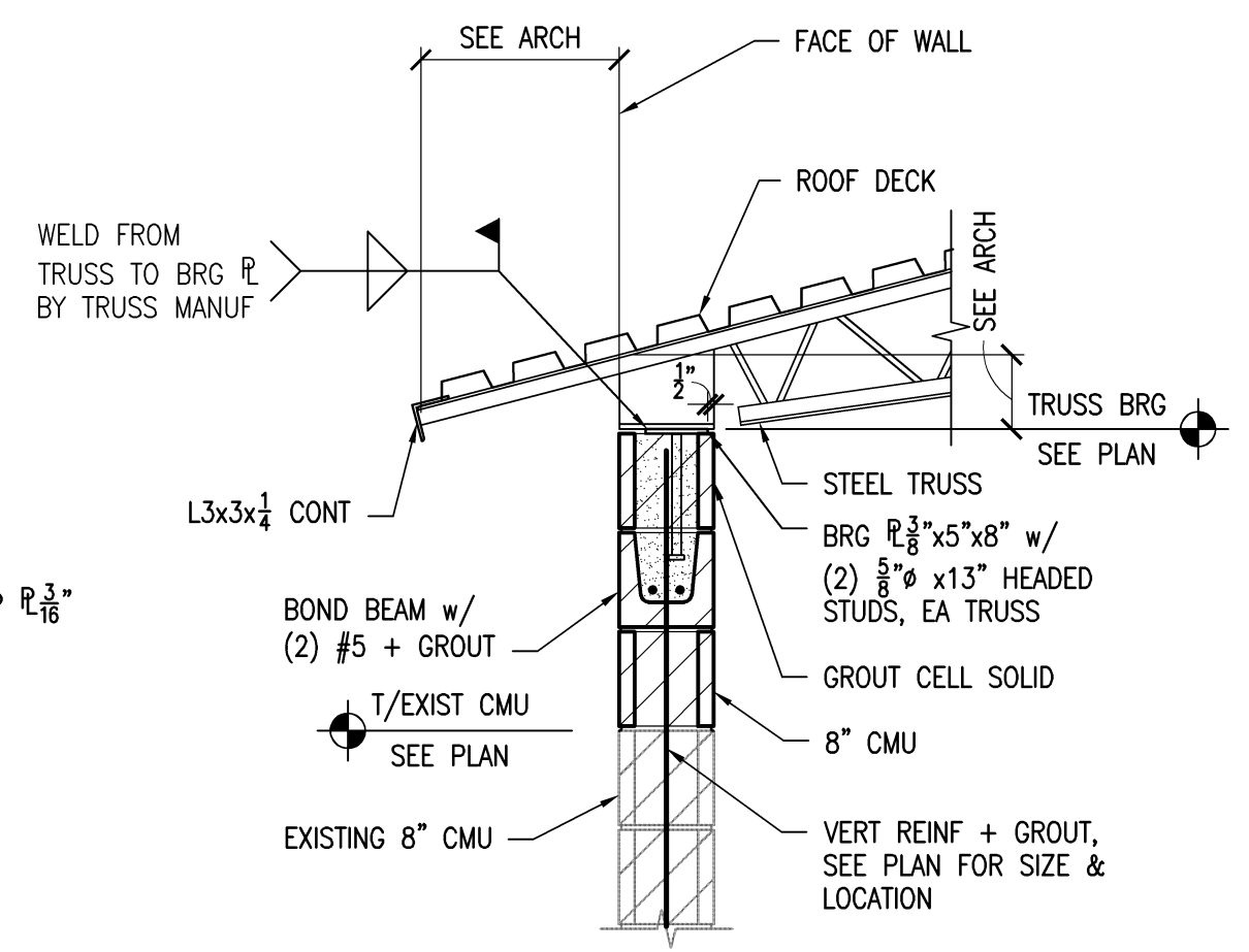
SECTION 9 3/4"=1'-0" S-4
