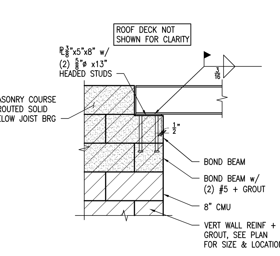
SECTION 4 3/4"=1'-0" S-4
