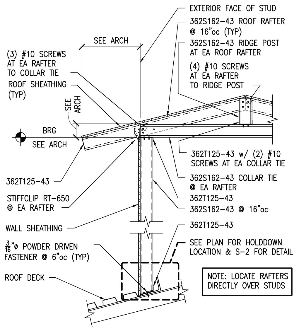
SECTION 6 3/4"=1'-0" S-4
