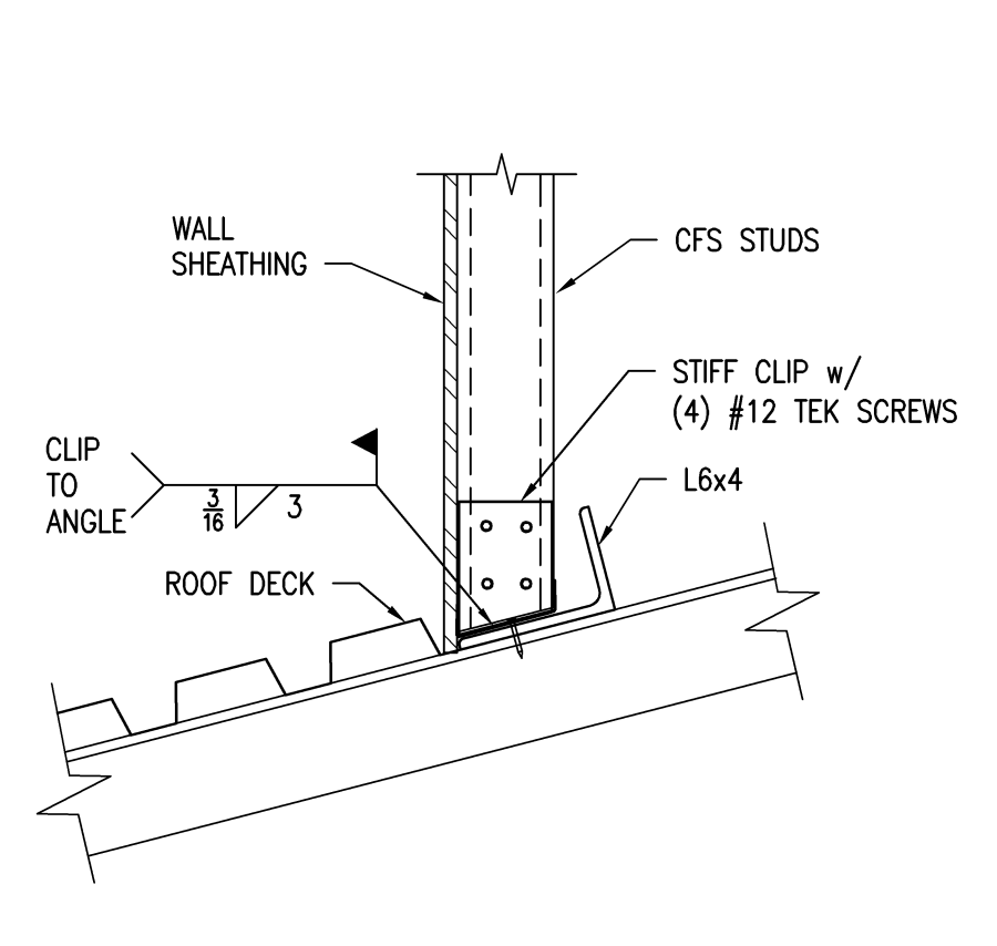
TYPICAL COLD FORMED STEEL HOLDDOWN 1 1/2"=1'-0"
