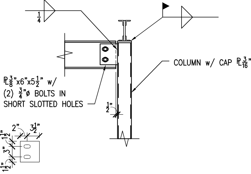
SECTION 8 3/4"=1'-0" S-4
