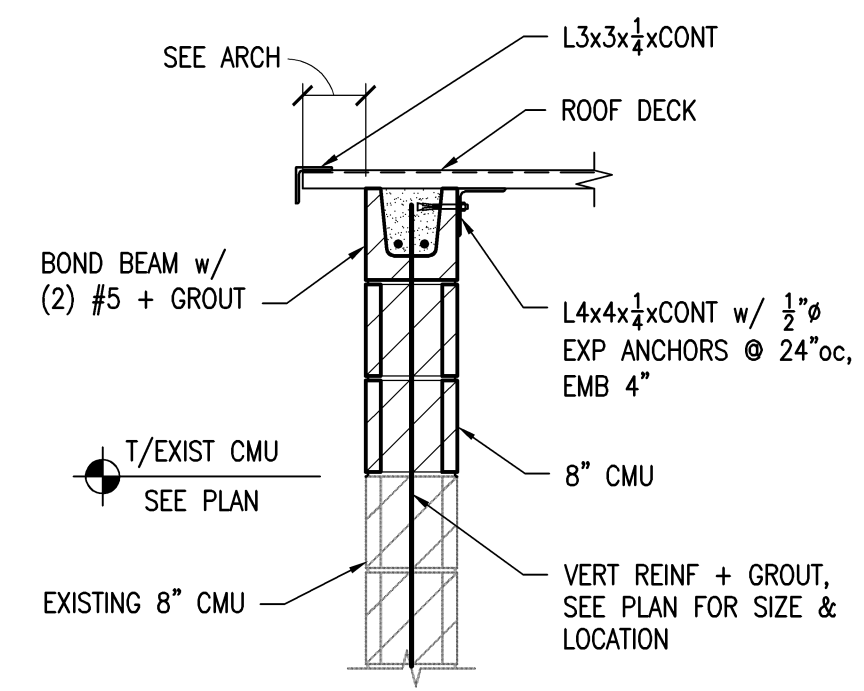
SECTION 10 3/4"=1'-0" S-4
