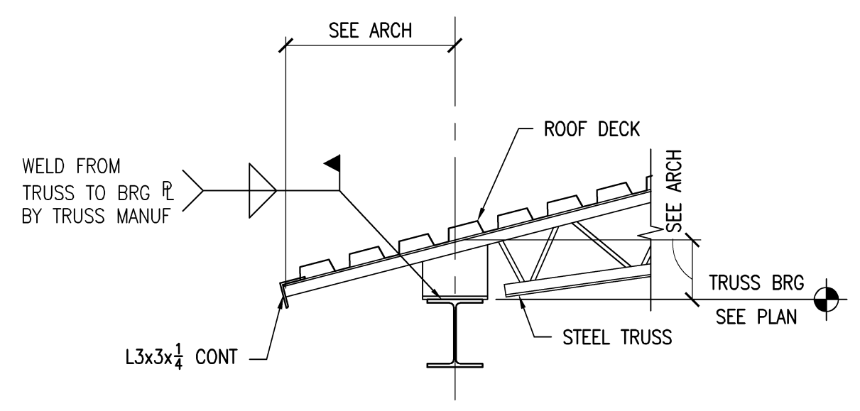
SECTION 12 3/4"=1'-0" S-4
