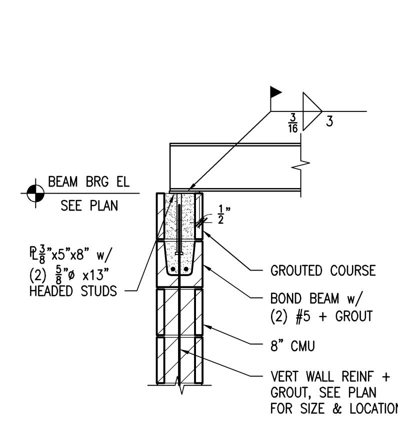
SECTION 3 3/4"=1'-0" S-4
