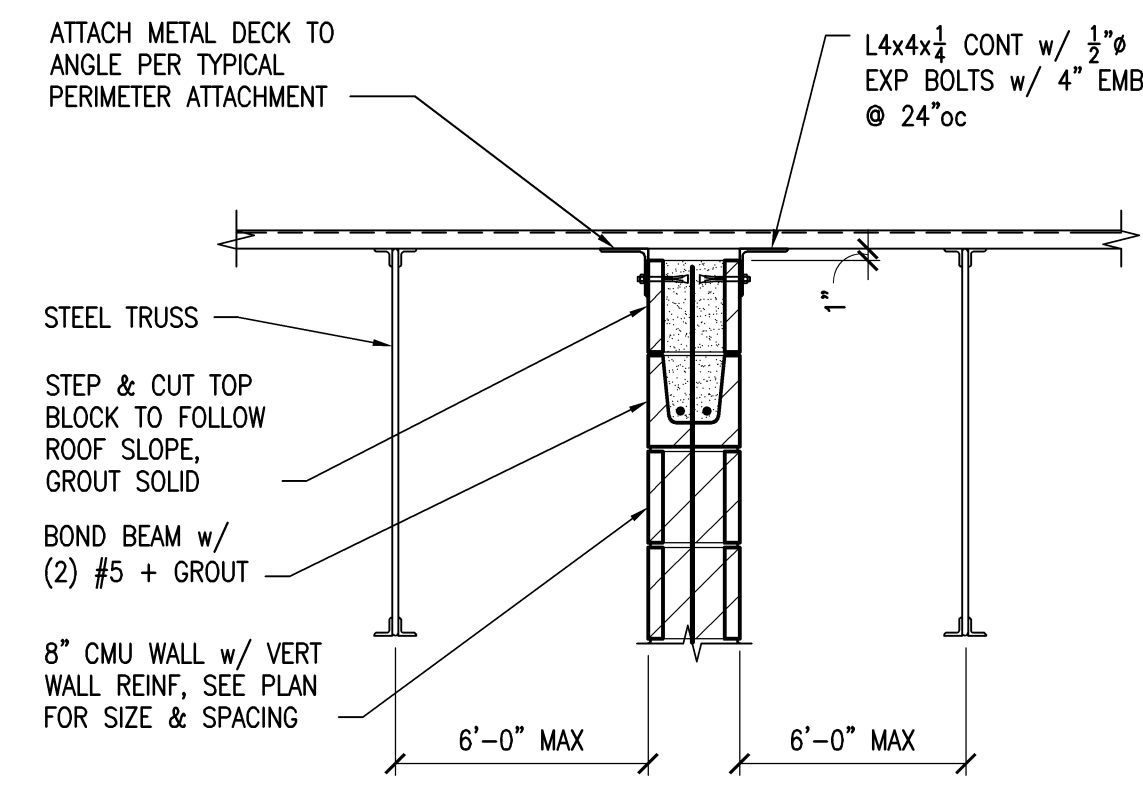
SECTION 7 3/4"=1'-0" S-4
