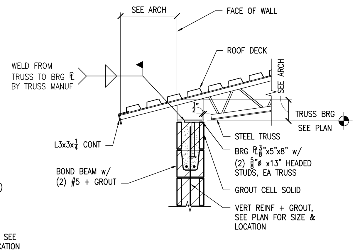
SECTION 2 3/4"=1'-0" S-4
