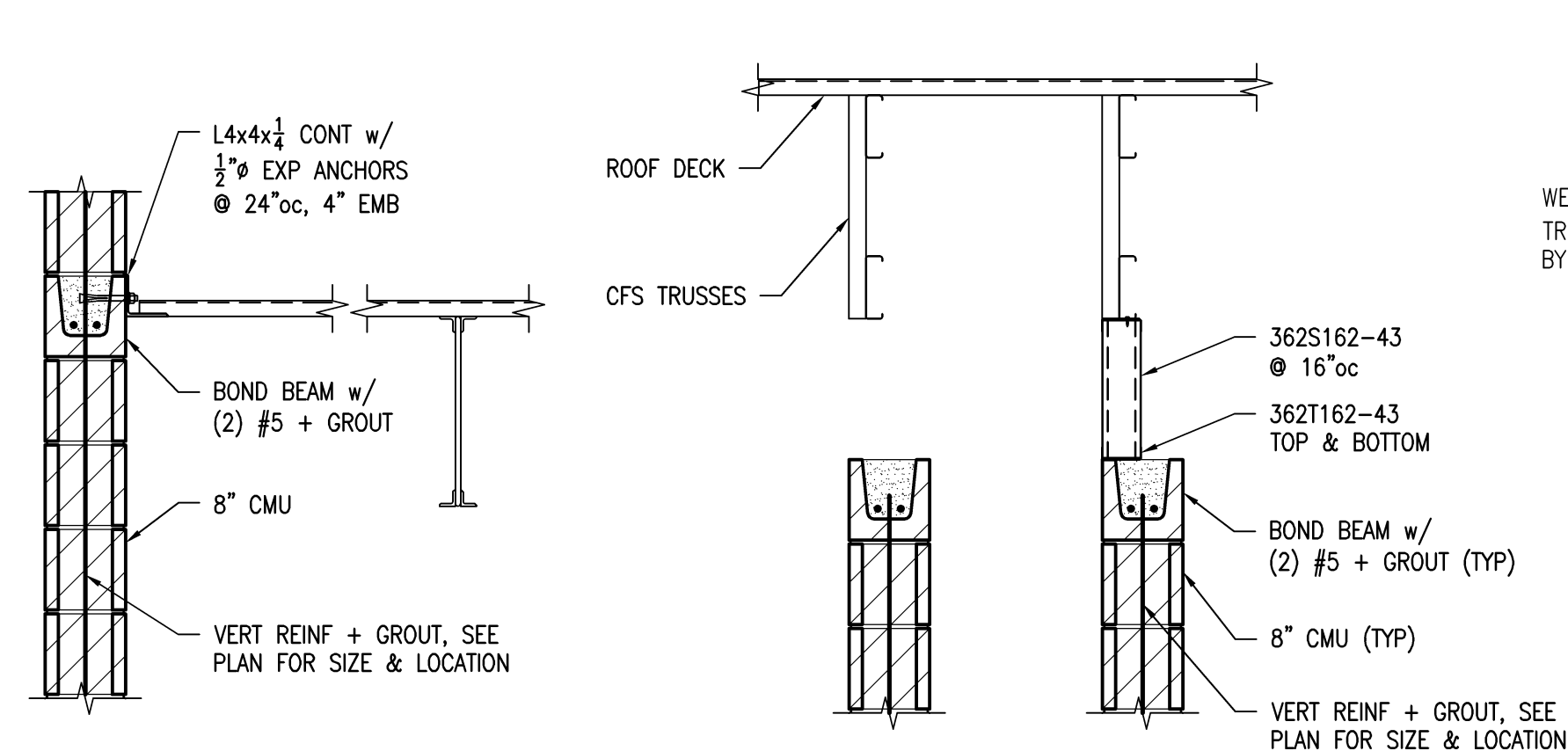
SECTION 1 3/4"=1'-0" S-4
